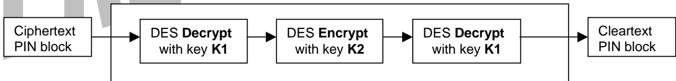
Diagram 2 - 3DES Decryption
